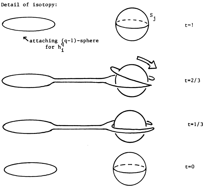
FIGURE 2c. Realizing T_{ij} (continued)
