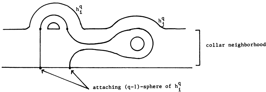
FIGURE 2b. Realizing T_{ij}
