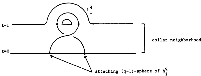
FIGURE 2a. Realizing U_i
